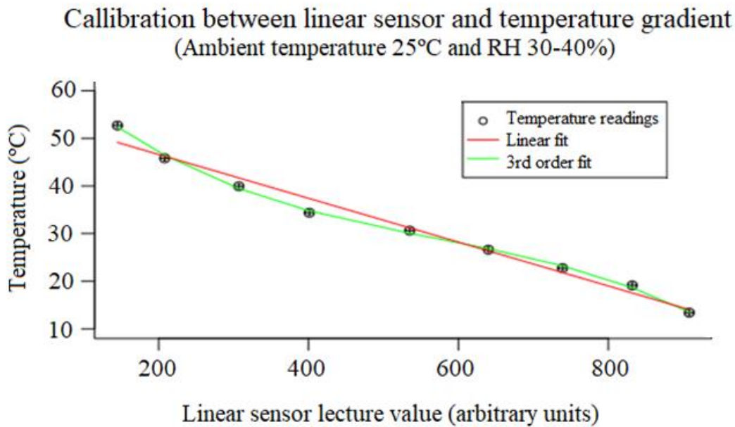
Figure 3. Linearity check of the temperature gradient along the metal bar. The x-axis represents the position on the linear sensor. This sensor is parallel to the metal bar, so the real length or position on the bar are not required to perform the mapping (Arduino analog-to-digital readings use 10 bits to store the readings —10 bits are 2^{10} , from 0 to 1024 values). The y-axis represents the local temperature in Celsius degrees (°C). This was performed at a standard room temperature of 25°C and with a relative humidity of 30-40%.
