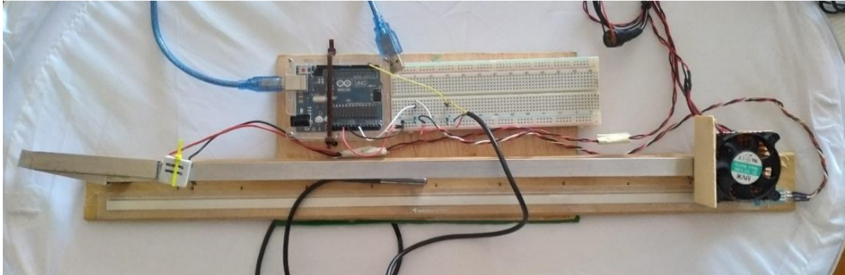
Figure 2. Termosensimetro prototype. Thermal stimulator that produces a thermal gradient along the grey metal bar. The thermal gradient is produced by Peltier modules at both ends of the grey metal bar. The tactile sensor is the white band below the metal bar.
